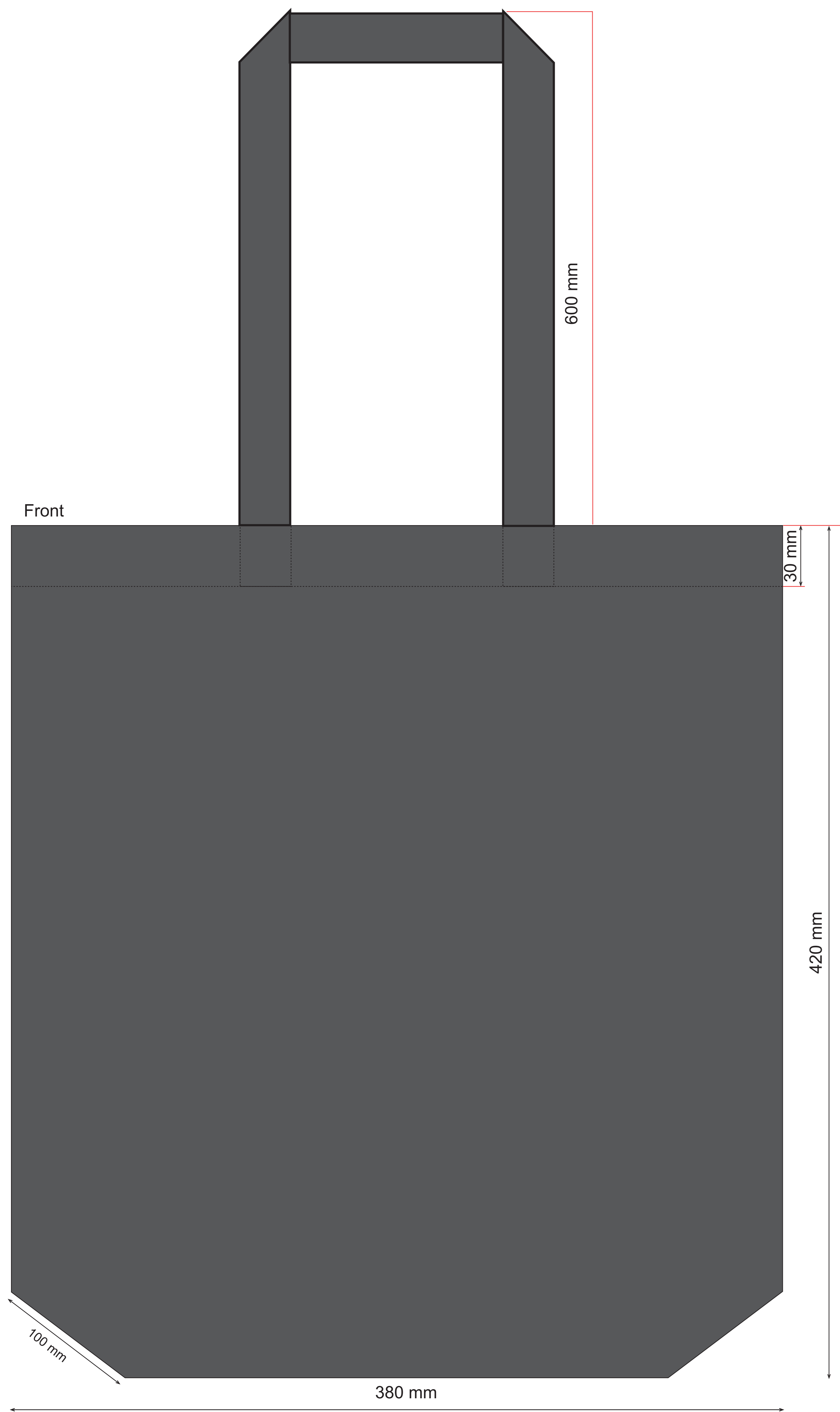
Bottom Guesset
